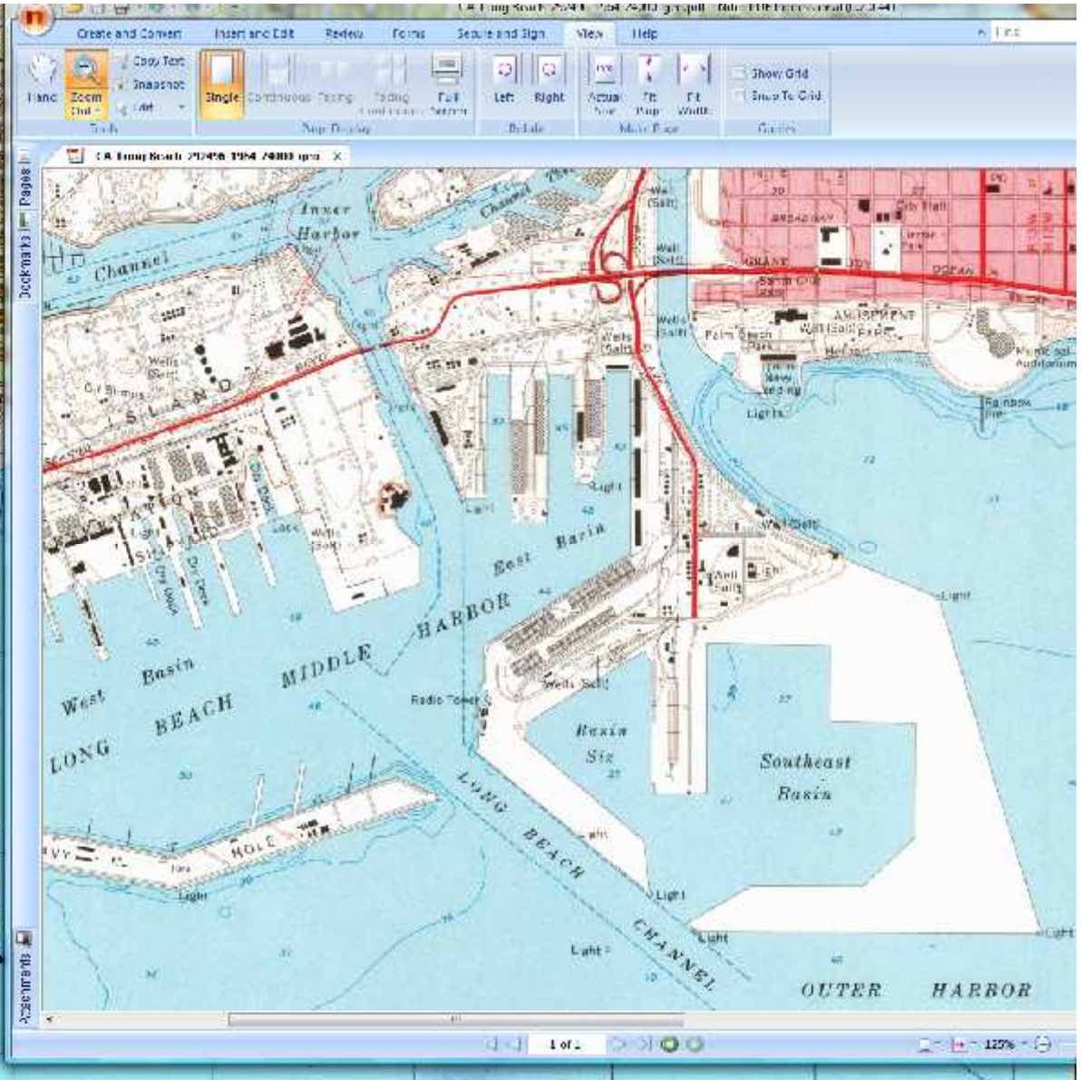
Los Angeles - Long Beach. Note differences such as shape of Southeast Basin and surrounding roads and storage tanks, buildings by Basin Six, bridge, roads and coastline by Rainbow pier, Seaside Blvd roads and bridges. Bathymetric depths do not correspond - 35ft in Basin Six is not 16m, 52ft in Inner harbour is not 17m.
